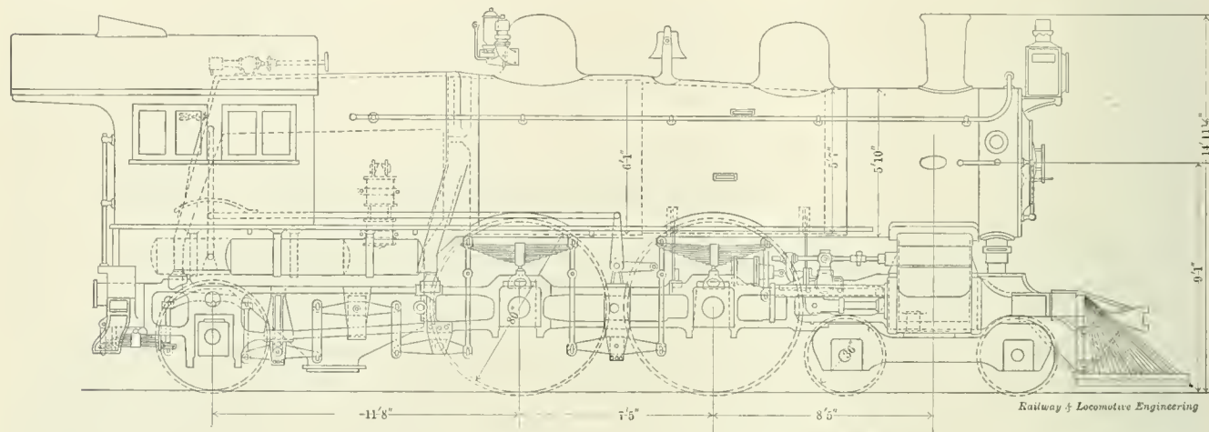
SIDE ELEVATION OF PENNSYLVANIA 4-4-2 PASSENGER ENGINE.
